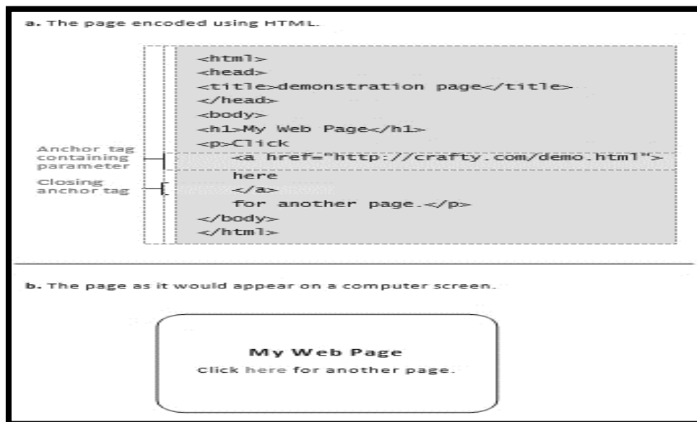
Figure 69: An enhanced simple webpage
