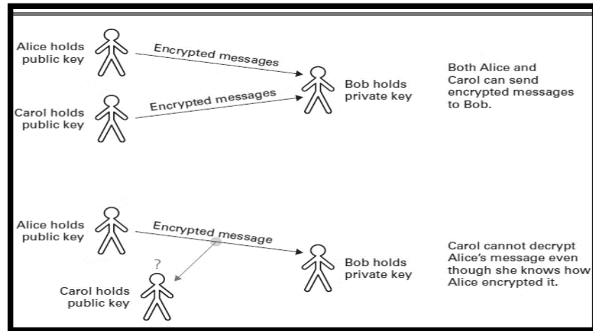
Figure 77: Public key encryption
