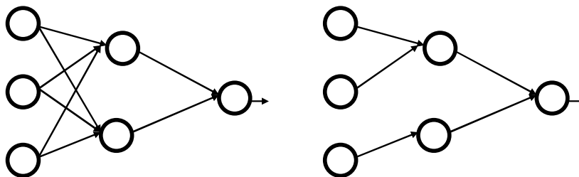
Fully connected
