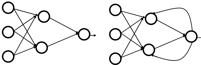
Feed forward
