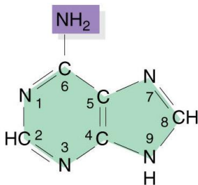
Adenine (A)
