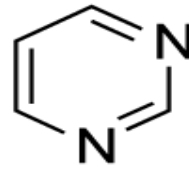
pyrimidine
