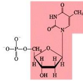
Deoxythymidine
