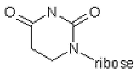
dihydrouridine
