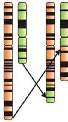
Translocation
