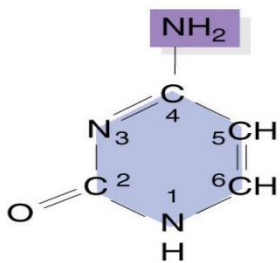
Cytosine (C)
