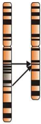
Deletion
