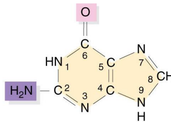
Guanine (G)
