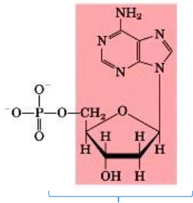
Deoxyadenosine
