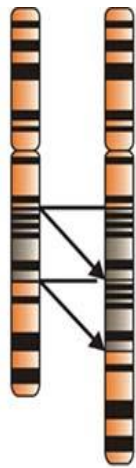
Duplication
