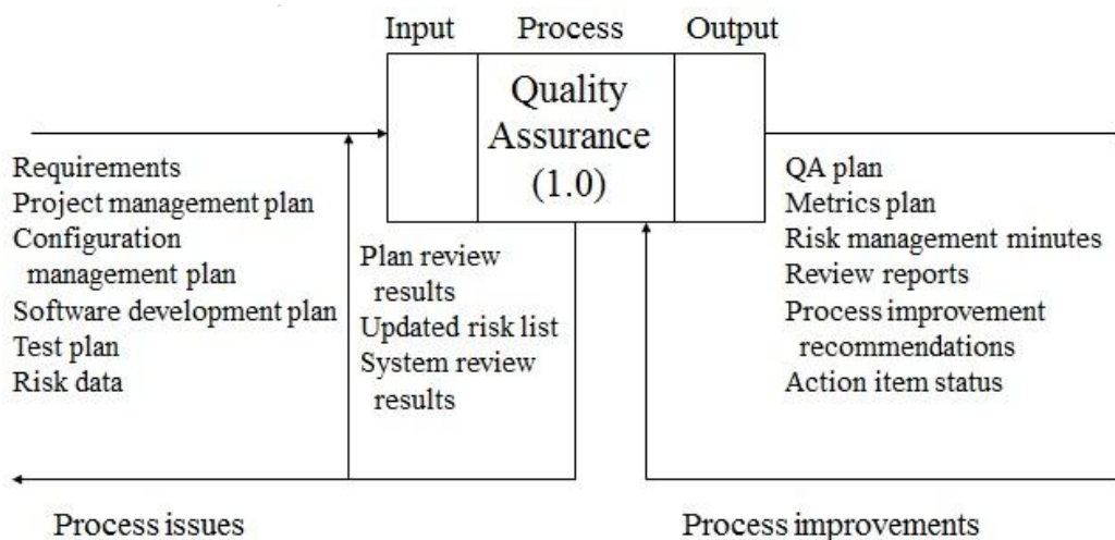
Software Quality Assurance Level 0 IPO Diagram
